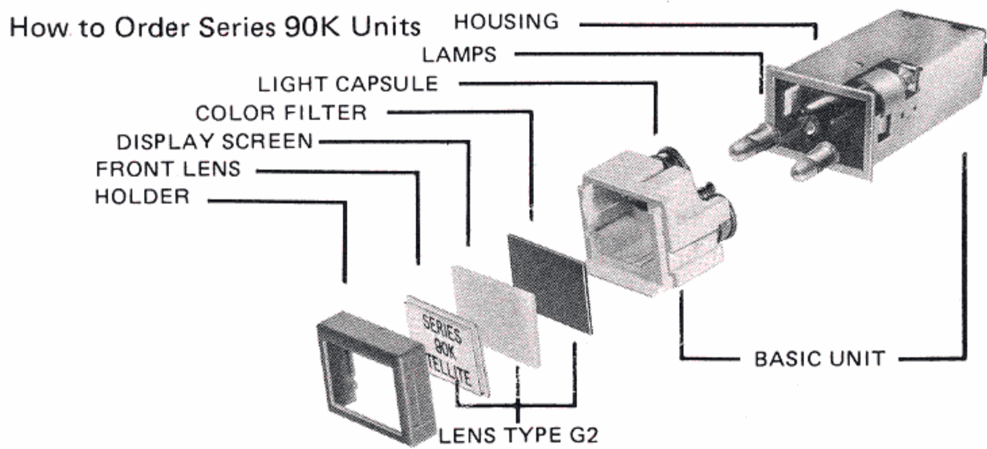
Component parts of a complete indicator unit (type G2 lens assembly shown).
