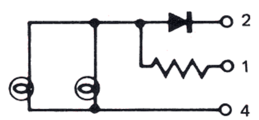
Control Circuit E9 Test & Diode Dimming D.C. Positive Input (For D.C. Negative Input specify E16)
