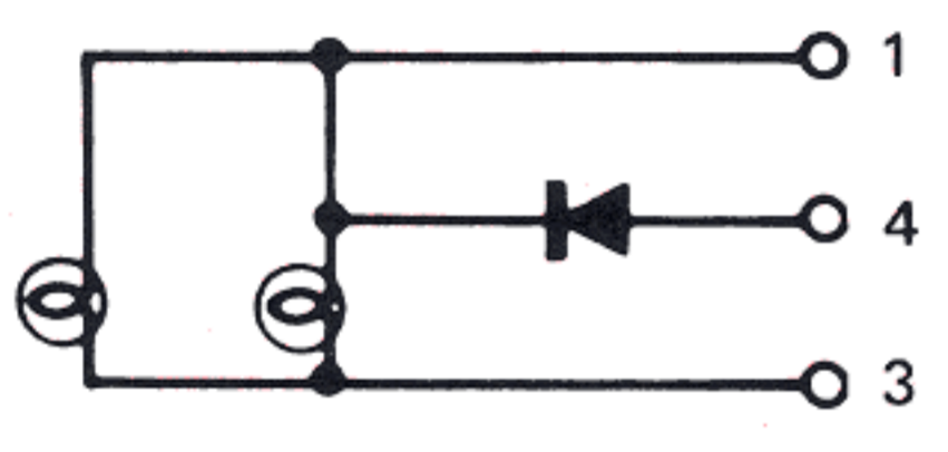
Control Circuit E5 Test D.C. Positive Input (For D.C. Negative Input specify E12)
