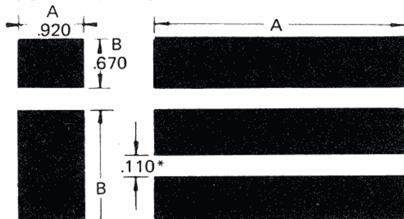
The panel cutout shown may be used for both housings shown above.
