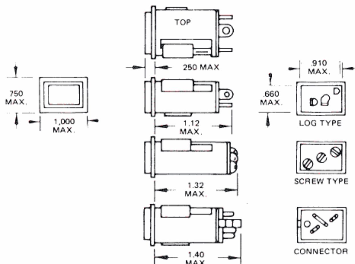
Outline dimensions to be used for Indicator-Lite and Press To Test.
