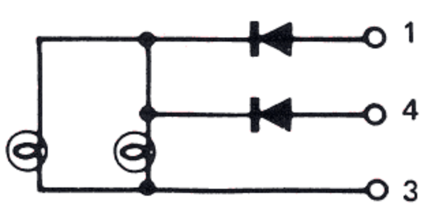
Control Circuit E6 Test With Blocking Diode D.C. Positive Input (For D.C. Negative Input specify E13)
